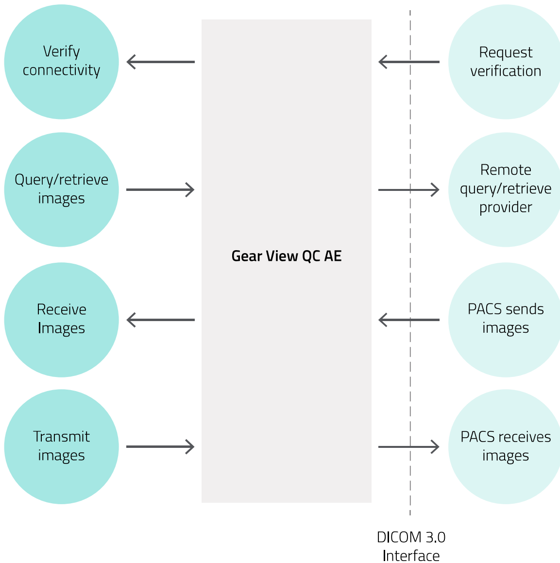
Figure 1. Gear View QC Implementation Model
